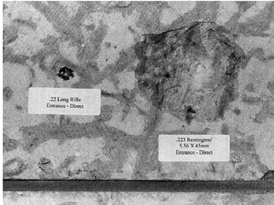
Figure 5 - Damage to Tindlestone Caused by .223 Remington
