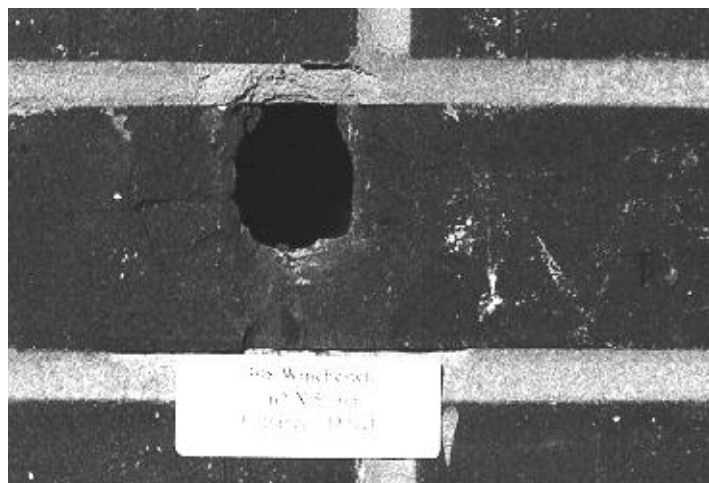
Figure 4 - Damage to High Strength Clay Brick Caused by .308 Winchester
