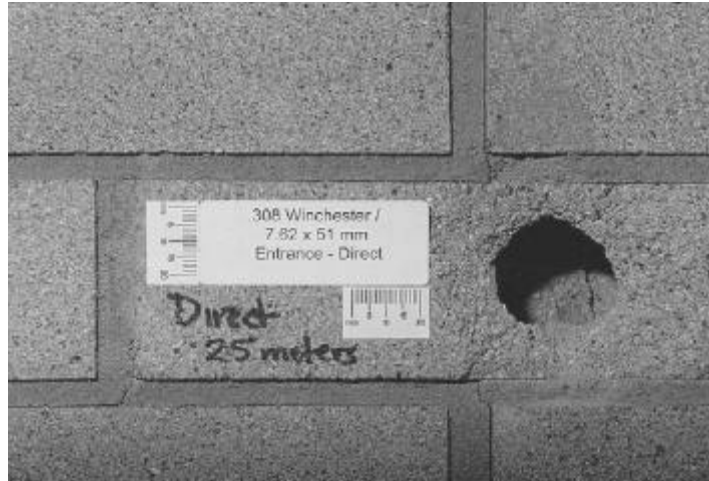
Figure 3 - Damage to Low Strength Clay Brick Caused by .308 Winchester
