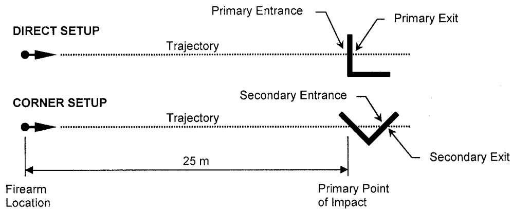
Figure 2 - Plan View of Test Setup
