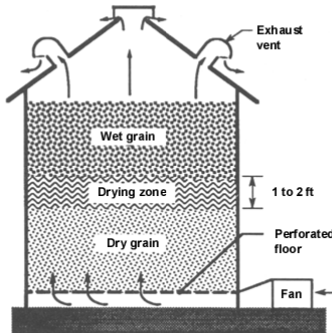
Figure 1. Schematic of natural-air drying bin.
