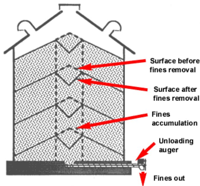
Figure 2. Removing fines during bin filling.
