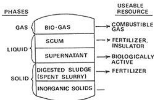
FIG.2 Layering of By-Products In the Digester
