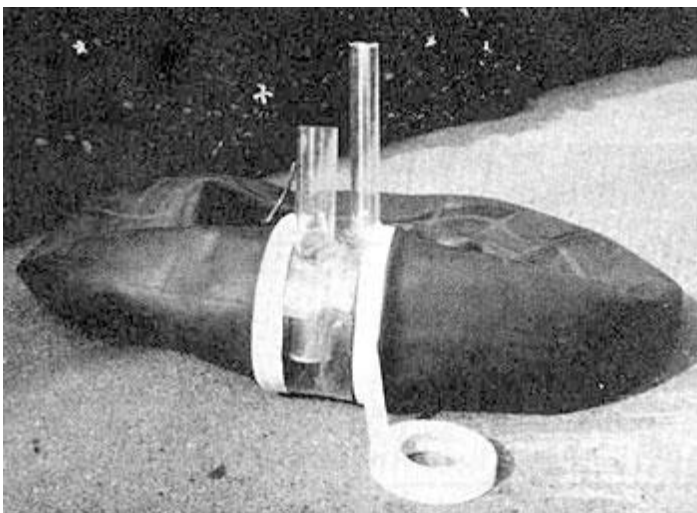
Fig. 26 Fastening tube to plexiglass cylinder
