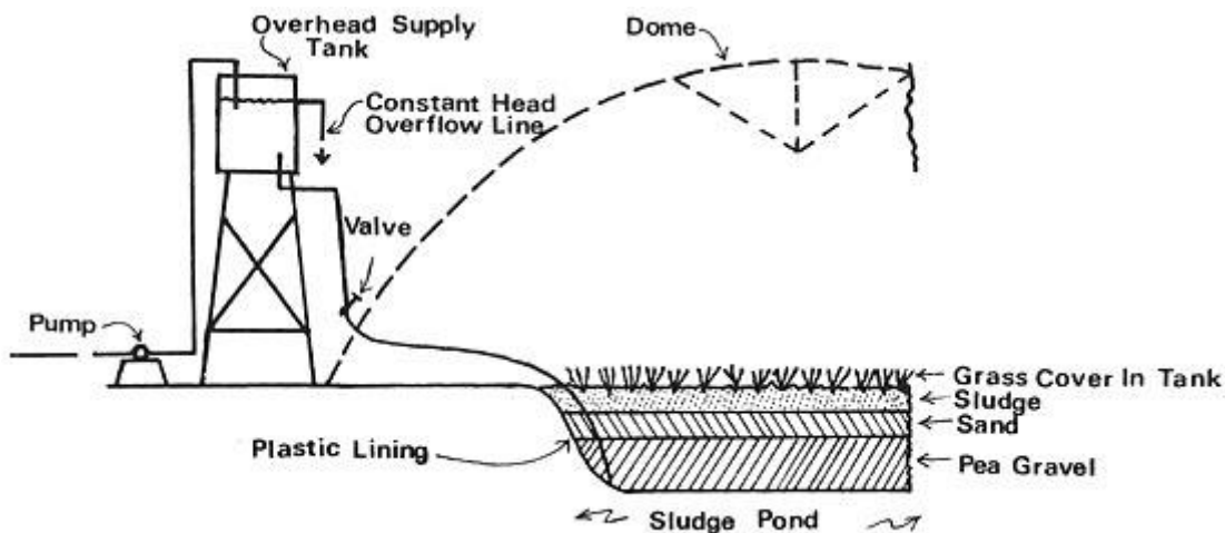
Fig. 16 Hydroponic sludge culture of pasture grasses
