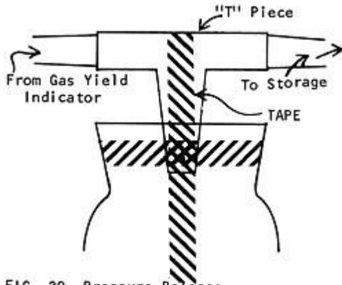
FIG. 29 Pressure Release
