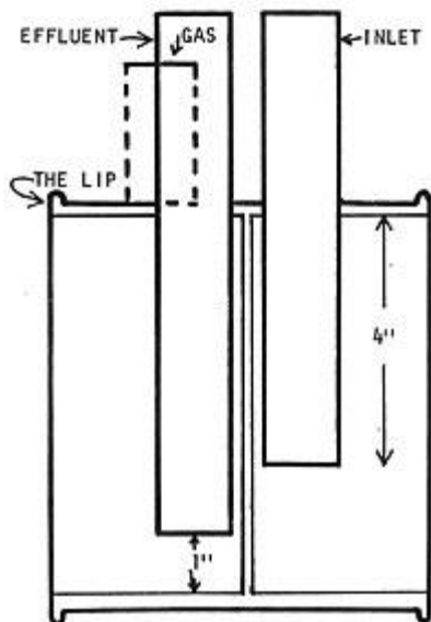
Fig. 23 Cross section of the plastic insert
