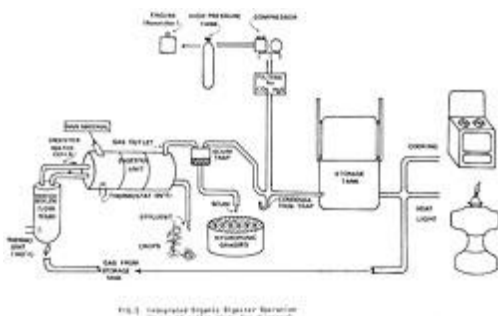
Fig. 5 Integrated organic digester operation (using 50 gallon drums for
