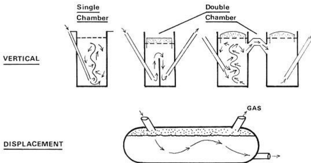
FIG.13 Types of Continuous-Feeding Digesters
