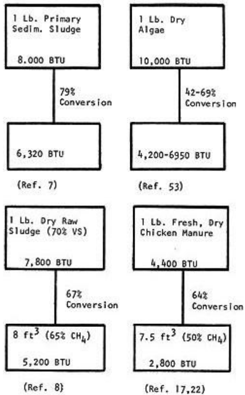
FIG.15 Efficiency of Methane Production from Different Materials
