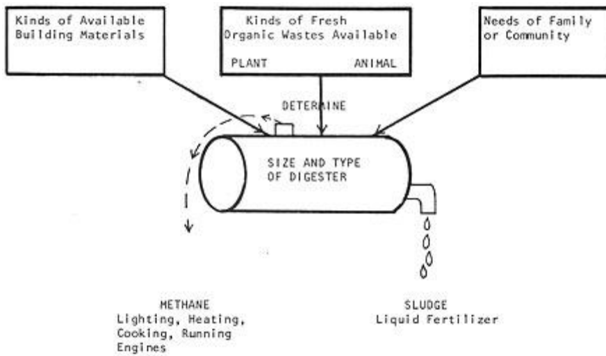
Fig. 3 Related considerations of a digester operation
