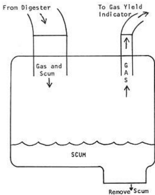
Fig. 27 Scum collector
