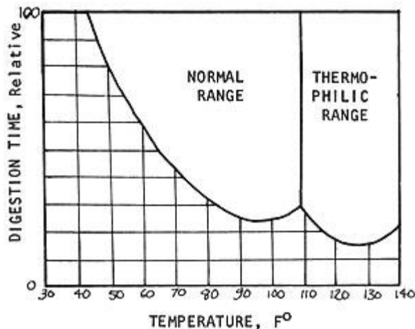
FIG. 8 Digestion Time and Temperature (after Ref. 7)
