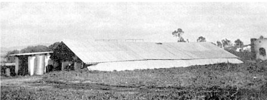
Engine room, summer cooling tank and digester on the first full scale methane power plant to operate on the linear displacement principle. Water heating tower on right was abandoned in the first year.
