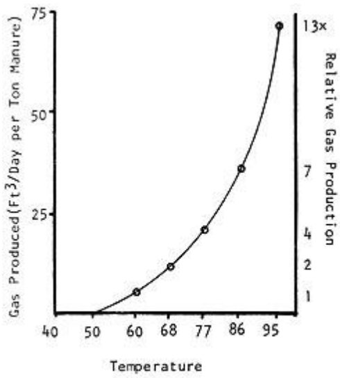
FIG.9 Gas Production and Temperature (after Ref. 15)
