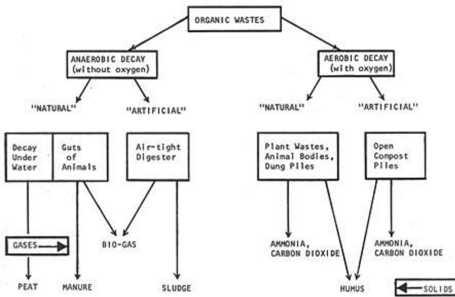
FIG.1 End Products of Organic Decay
