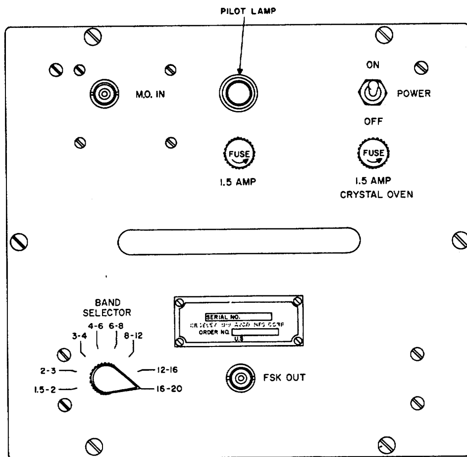
Figure 3-1. Modulator, Radio MD-239(*)/GR, front panel controls.
