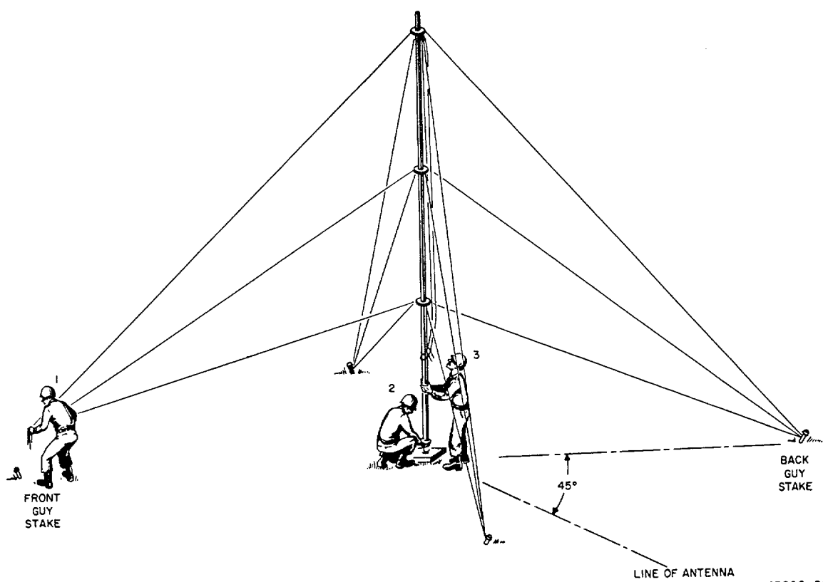
Figure 2-4. Revising assembled Mast AB -155(*)/U.
