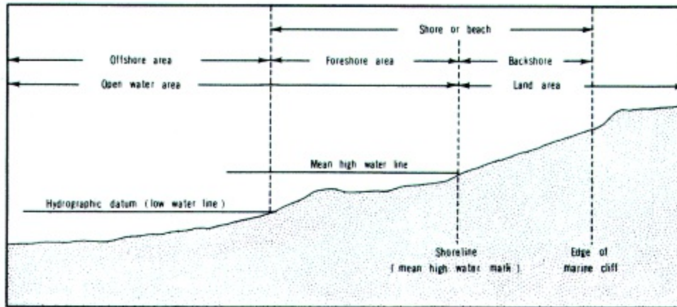
Figure 82. Definition of Coastal Terms.
