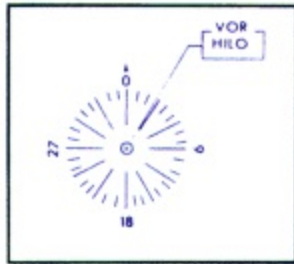
Figure 272. OMNI Range (Omnidirectional Range). Identified as VOR (very high frequency omnidirectional range), VORTAC (very high frequency omnidirectional range Tactical Air Command), or TACAN (tactical air navigation). The compass rose (magnetic bearing circle) is oriented to magnetic north and centered on the station. Name of the facility is shown in rectangular box.
