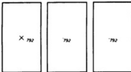
Figure 230. Non-monumented Bench Mark. (sometimes called temporary, supplementary, or intermediate). The symbol represents a described vertical control point which was established by survey methods of third or higher order accuracy. The point is usually recoverable. The mark does not bear a tablet.
