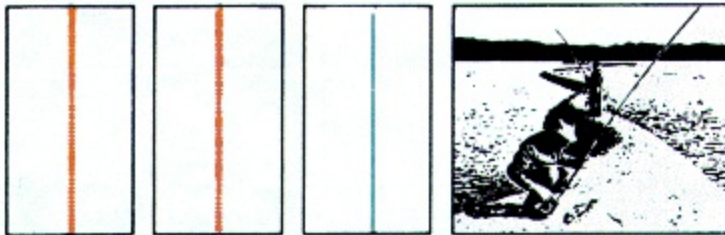
Figure 51. Small Levee. Large levees are shown by contours, except in extremely flat areas.
